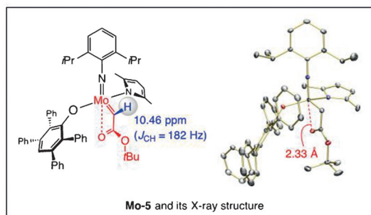
Scheme 2. Preparation and structural analysis of two ester-substituted Mo alkylidene complexes.
