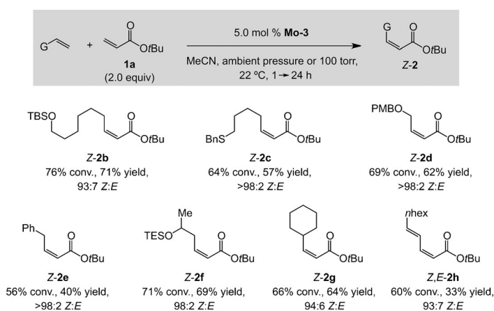
Scheme 3. ( Z )- \alpha,\beta -Unsaturated esters obtained through catalytic cross-metathesis. Reactions performed at 100 Torr for 1 h ( 2b,c ), at 100 Torr for 4 h ( 2d–f ) and at ambient pressure for 24 h ( 2g–h ). See the Supporting Information for details.
