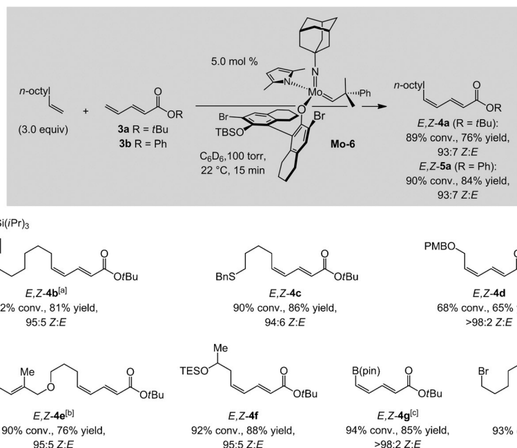
Scheme 4. ( E,Z )-Dienoates obtained through catalytic Z -selective cross-metathesis. [a] Overall yield after removal of the silyl group. [b] 1.5 equiv 1-decene used. [c] Reaction time = 24 h. See the Supporting Information for details.
