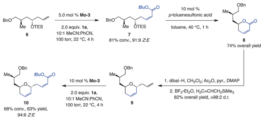
Scheme 5. Application to stereoselective synthesis of the C1-C12 segment of laulimalide.
